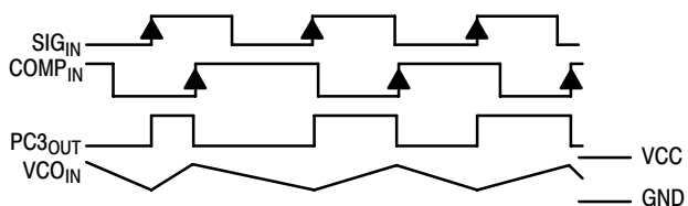
Figure 10. Typical Waveform for PLL Using Phase Comparator 3
