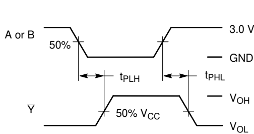
Figure 5. Switching Waveforms
