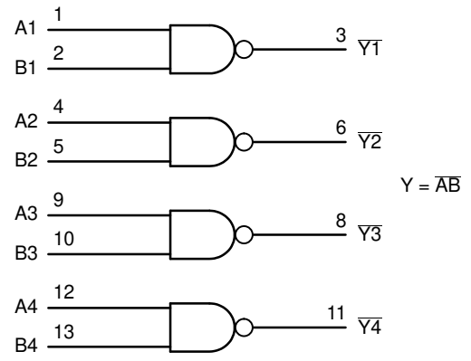
Figure 2. Logic Diagram
