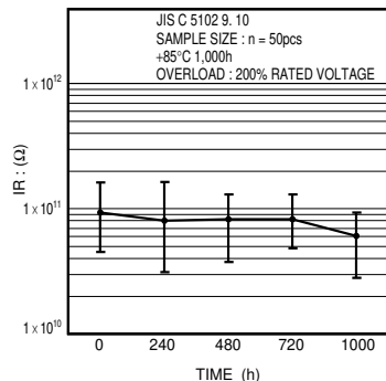
Fig.24 Insulation resistance
