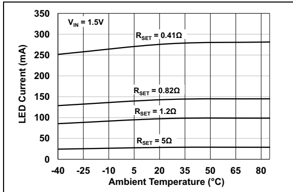
FIGURE 2-7: One White I_{LED} vs. Ambient Temperature.
