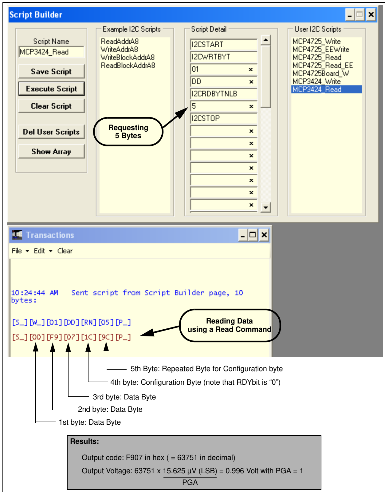
FIGURE 1-5: Reading Conversion Results: Note that the Input = 0.996V is applied at CH1. The reading indicates the measured value is 0.996 Volts.
