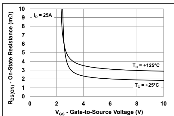
FIGURE 2-3: On Resistance vs. Gate-to-Source Voltage.
