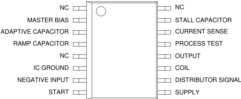
Figure 3. 33094 Pin Connections
