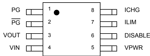
Figure 3. 8-SOICN Pin Connections
