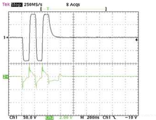
Figure 10: Typical Waveform
