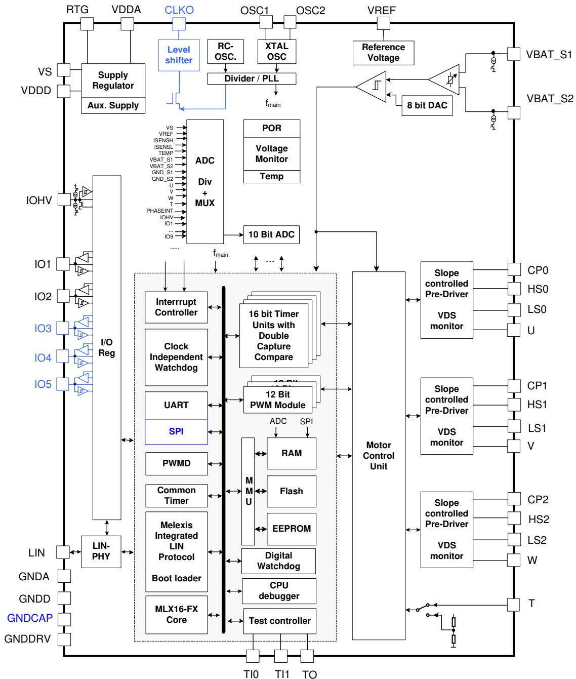
Figure 1 – Block Diagram
