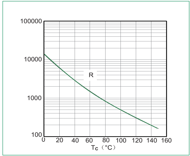
Figure 14: NTC Characteristics
