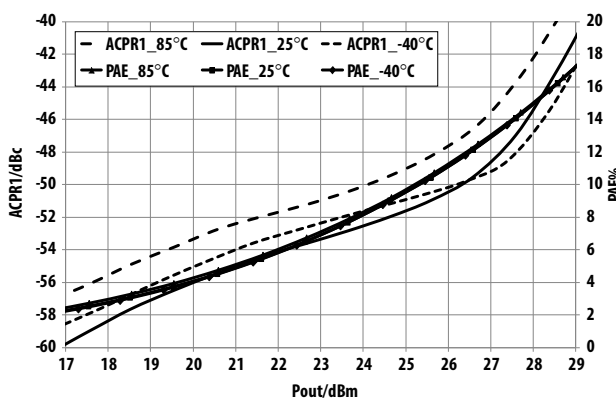
Figure 12. Over-temperature ACPR1, PAE vs. P_{out} @ 2.36 GHz V_{dd}=V_{ddBias}=5.0\text{ V} operating voltage
