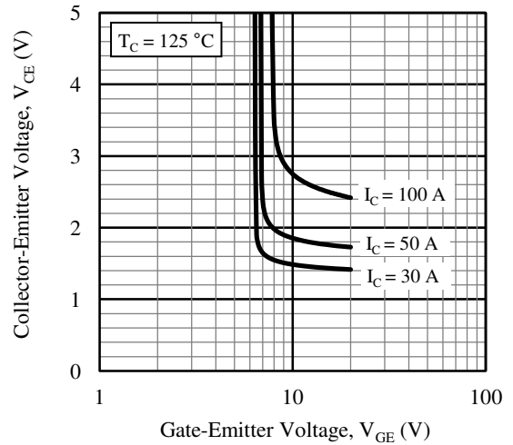
Figure 10. Collector-Emitter Voltage vs. Gate-Emitter Voltage
