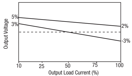
MGJ2D121505SC & MGJ2D241505SC
