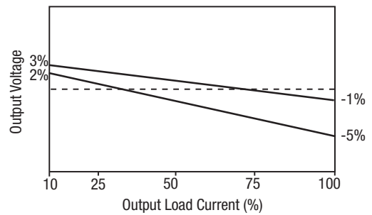
MGJ2D121505SC & MGJ2D241505SC
