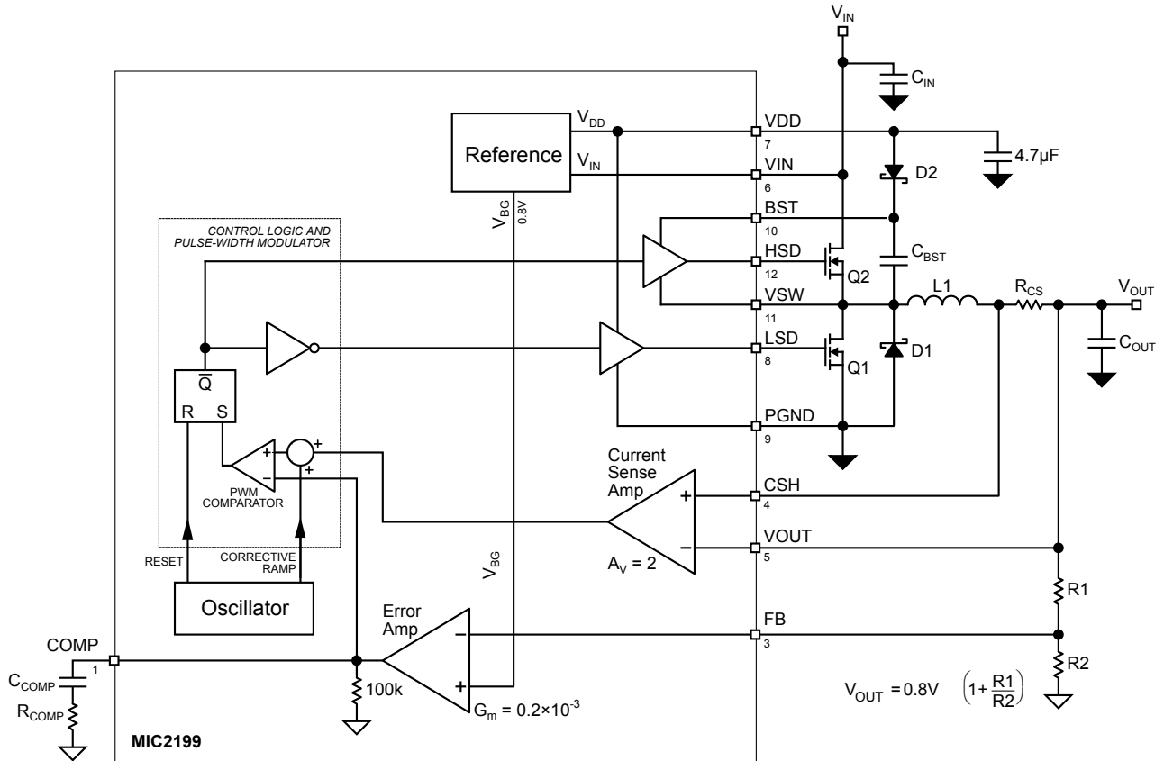
Figure 2. PWM Operation
