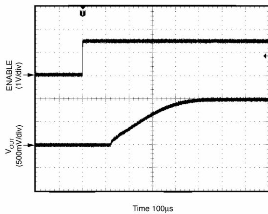
Turn-On Transient
