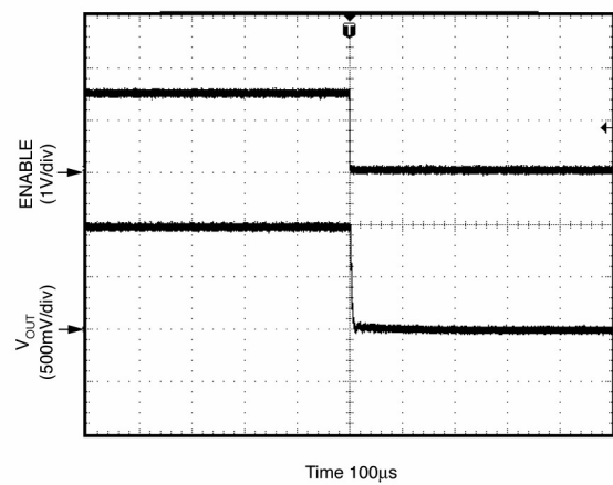
Turn-Off Transient
