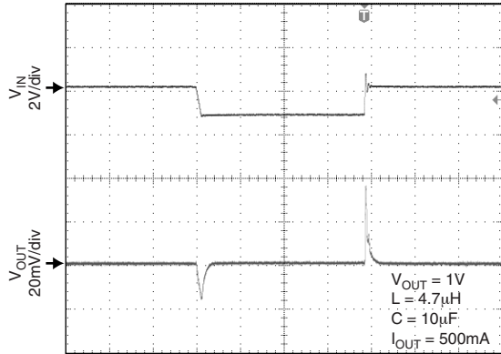
Line Transient
