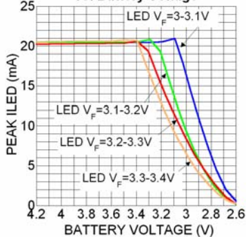
20mA Peak ILED vs. Battery Voltage
