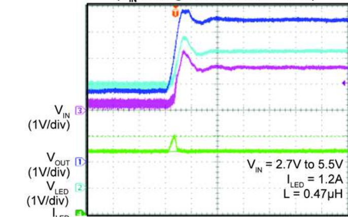
Line Transient (V_IN Changes from 2.7V to 5.5V)
