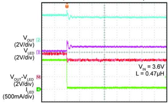
Load Transient (Flash 1.2A to Torch 63mA)
