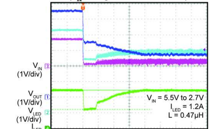
Line Transient (V_IN Changes from 5.5V to 2.7V)
