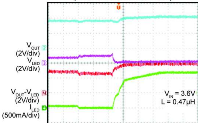
Load Transient (Torch 63mA to Flash 1.2A)
