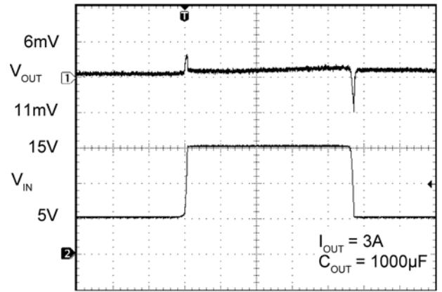
MIC29302A Line Transient Response with 3A Load, 1000µF Output Capacitance
