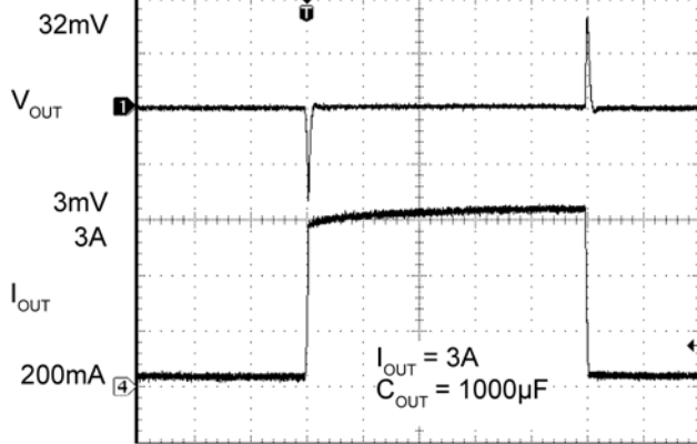
MIC29302A Load Transient Response with 3A Load, 1000µF Output Capacitance
