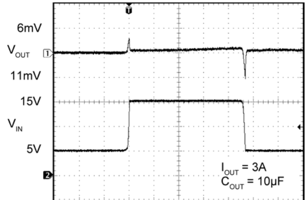
MIC29302A Line Transient Response with 3A Load, 10µF Output Capacitance
