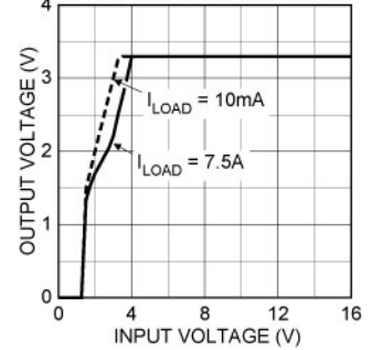
MIC29710-3.3 Dropout Characteristics
