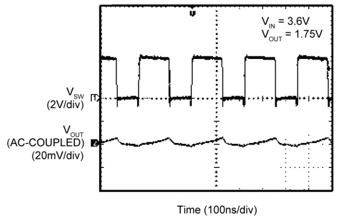
Switching Waveform Continuous Mode (1A)
