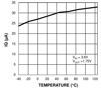
Quiscent Current vs. Temperature
