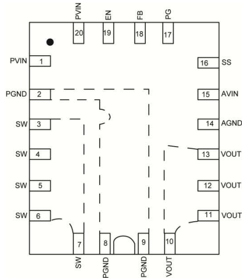
2.5mm × 3mm QFN (GK) (Top View)
