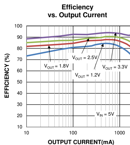
Figure 2. Efficiency under Load
