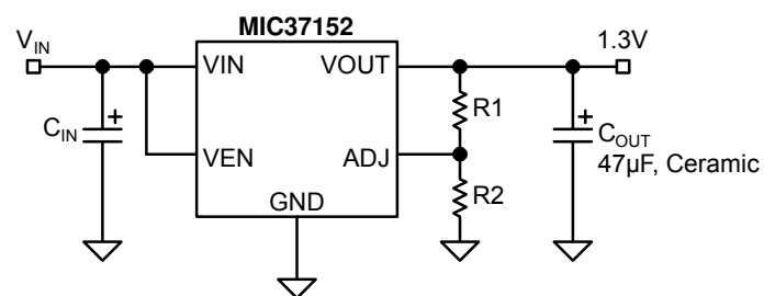
Adjustable Regulator
