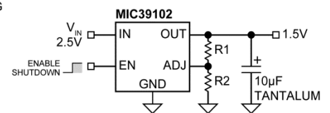
1.5V/1A Adjustable Regulator
