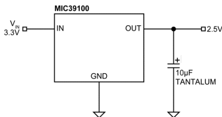
2.5V/1A Regulator
