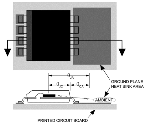
Figure 3. Thermal Resistance
