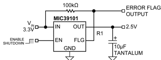
2.5V/1A Regulator with Error Flag
