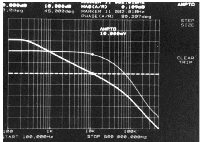
Figure 11. 3.3V/2A Output Bode Plot (θ Margin = 80°)
