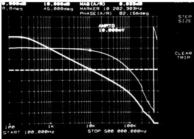
Figure 10. 3.3V/1A Output Bode Plot (θ Margin = 82°)
