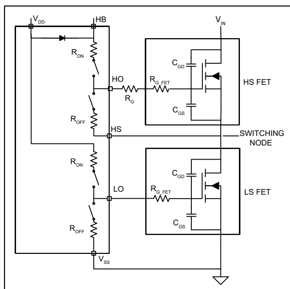
FIGURE 6-4: Gate Drive Circuit with Parasitics.
