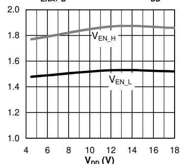
V_{ENA, B} Threshold vs. V_{DD}
