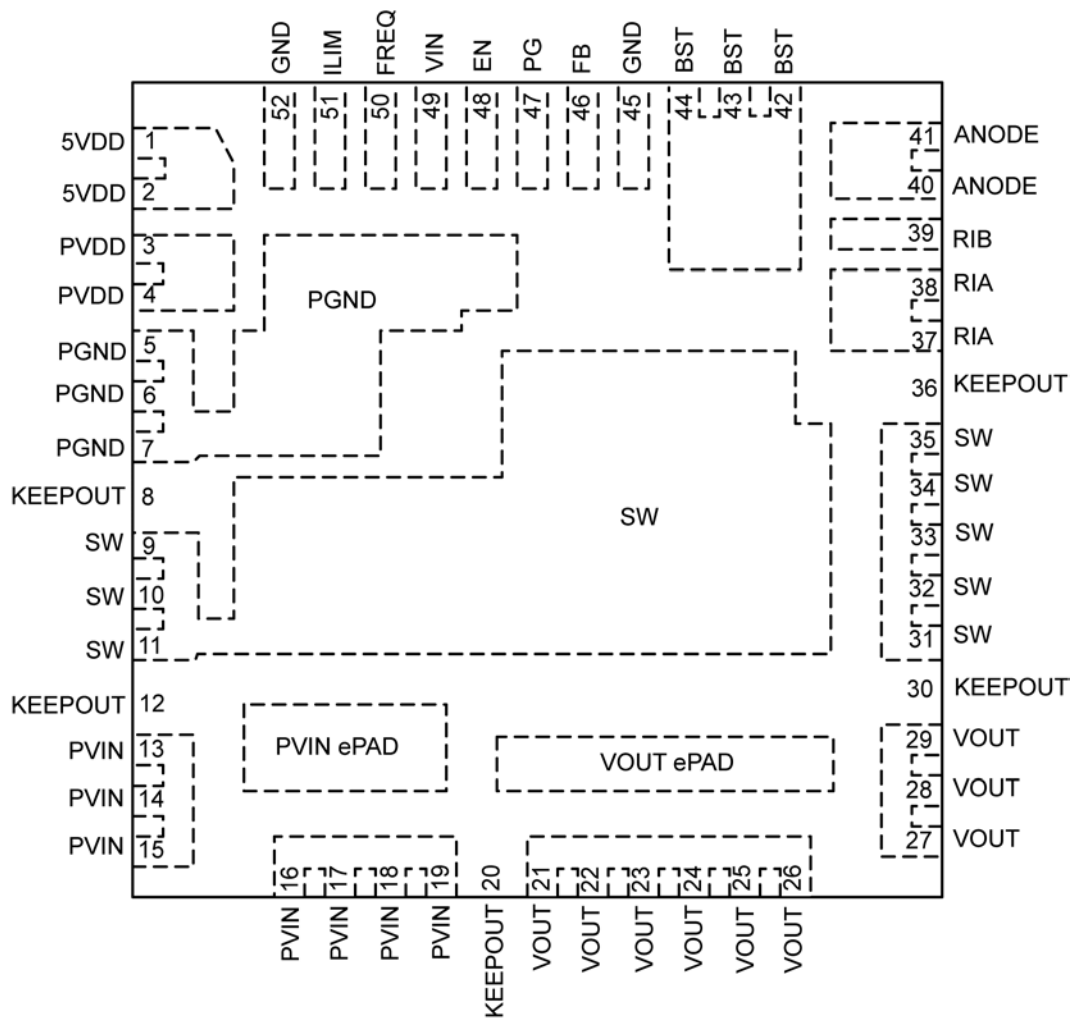
52-Pin 10mm × 10mm QFN (MP) (Top View)
