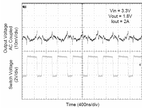
Output Ripple
