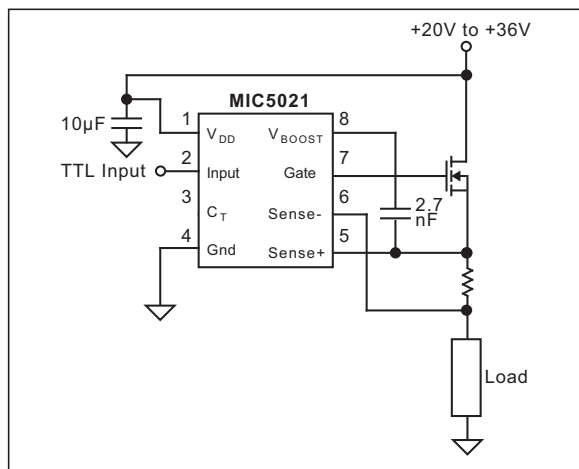
FIGURE 6-2: 12V to 36V Configuration.
