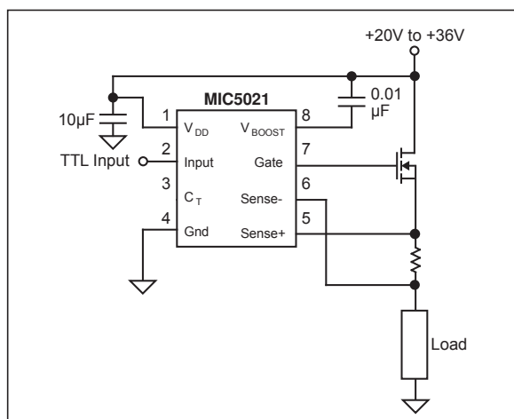
FIGURE 6-3: Preferred 20V to 36V Configuration.
