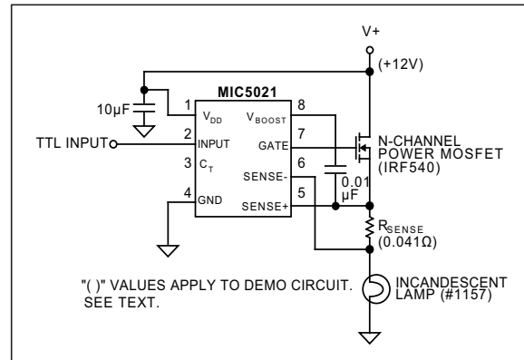
FIGURE 6-11: Lamp Driver with Current Sensing.
