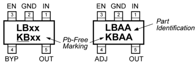
MIC5205-x.xBM5/YM5 Fixed Voltages
