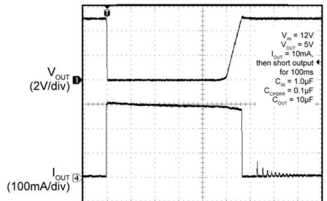
Current Limit
