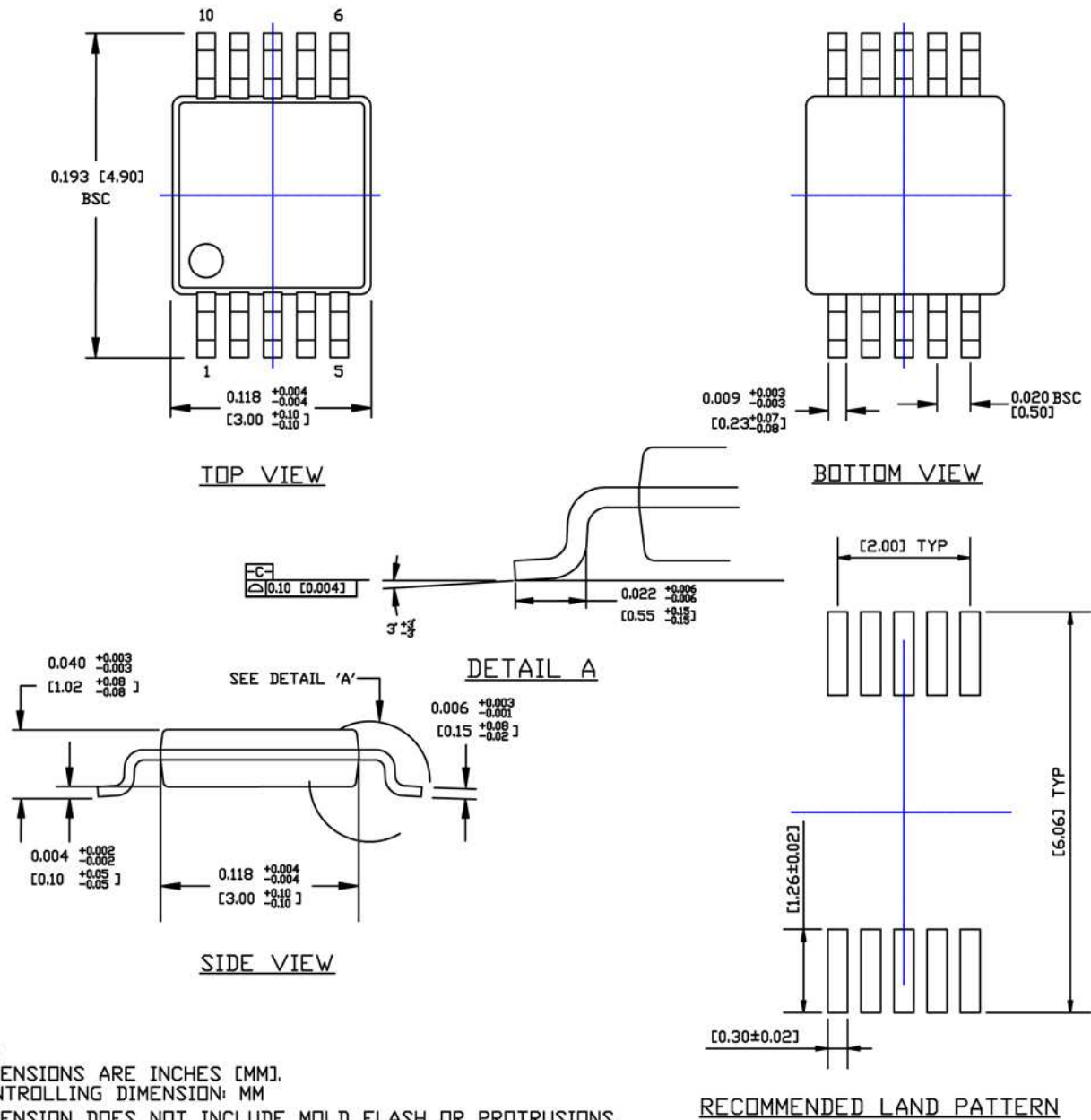
10-Pin MSOP (MM)
