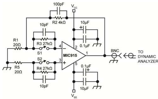
Noise Measurement
