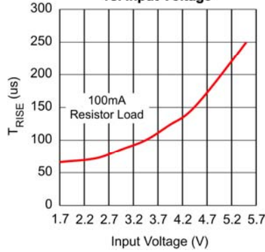
Rise Time vs. Input Voltage
