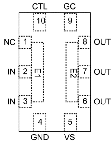
10-Pin 1.2mm × 2.0mm QFN (FL) (Top View)
