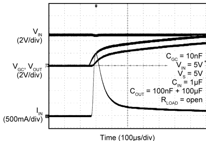
Figure 1. OUT voltage and inrush current waveform during turn-on (IN current scale is 500mA/div)
