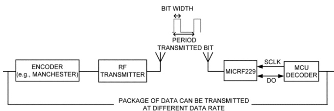
Figure 2. Transmitted Bit Rate through the Air
