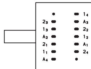
4 CIRCUITS 2 POSITIONS
