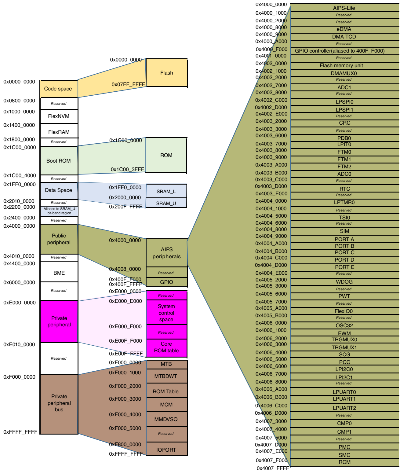
Figure 6. Memory map
