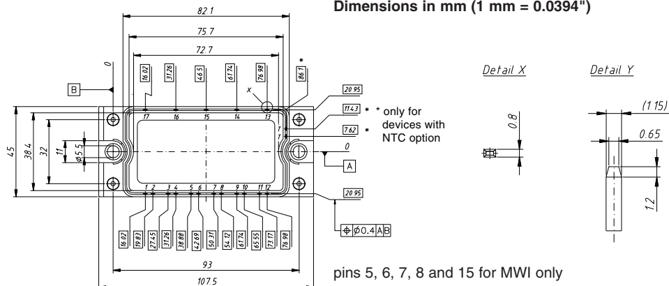
Dimensions in mm (1 mm = 0.0394")
