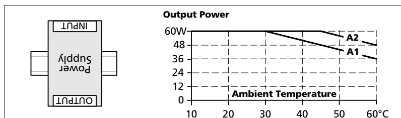
Fig. 22-8 Mounting Orientation B (Upside down)
