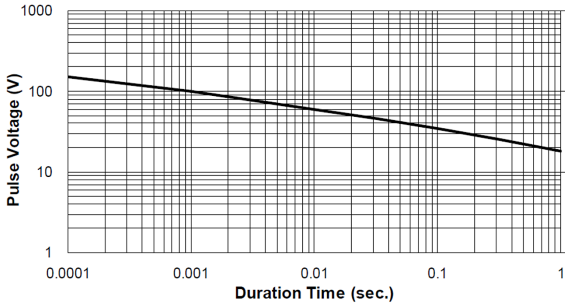
MLFA13 Pulse Voltage (100 Ohm)
