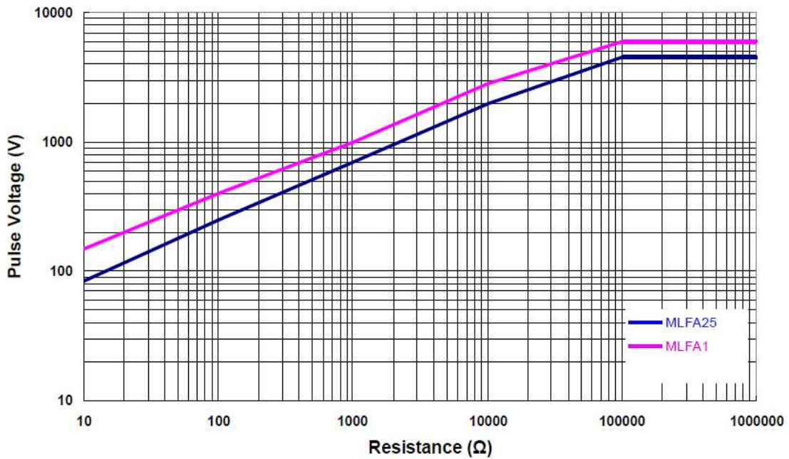
MLFA25/MLFA1 1.2/50 \mu s Lightning Surge
