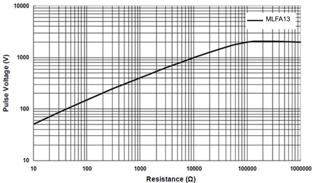
MLFA13 1.2/50µs Lightning Surge
