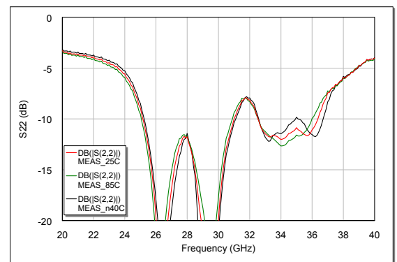
S22(dB)
