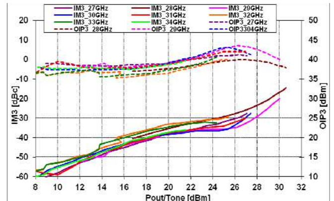
@ V_{ds}=5V , I_{dsq}=2.6A
