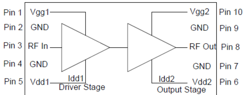
Figure 1 Functional Diagram
