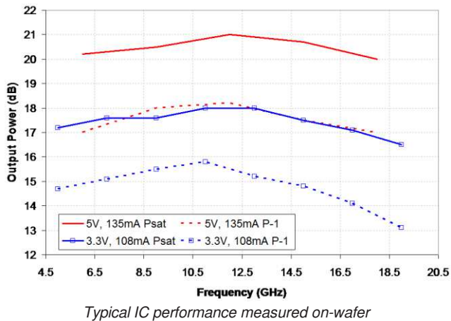
Output Power
