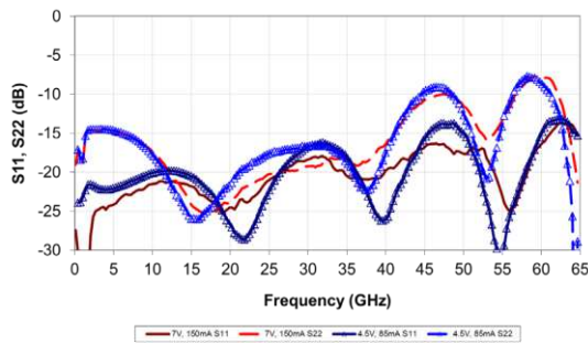
Typical IC performance measured on-wafer
