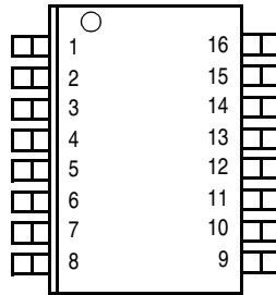
16-Pin SOIC Package N/C pins are recommended to be left FLOATING
