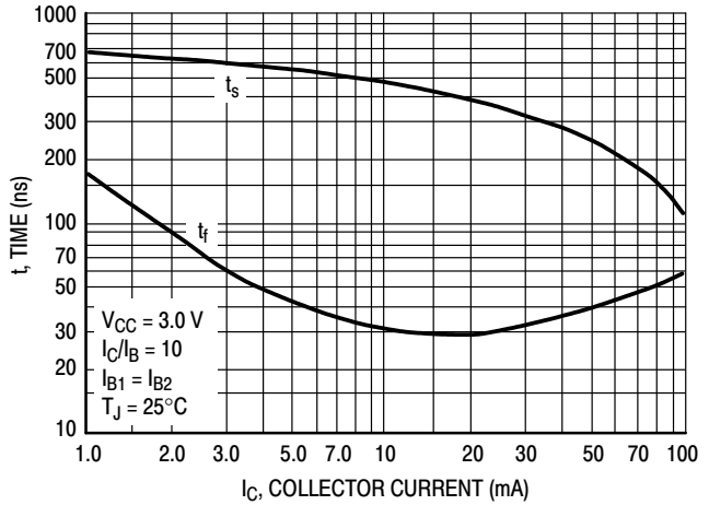
Figure 15. Turn-Off Time
