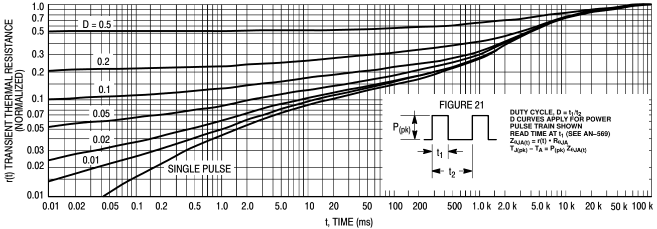
Figure 20. Thermal Response
