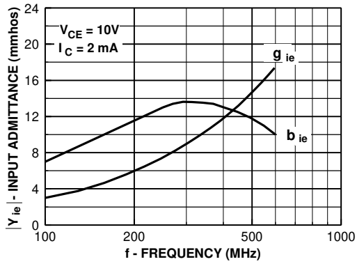
Input Admittance
