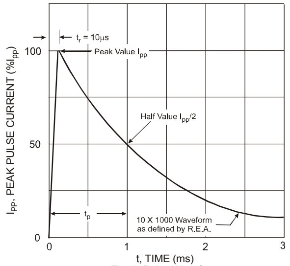
Fig. 2 Pulse Waveform
